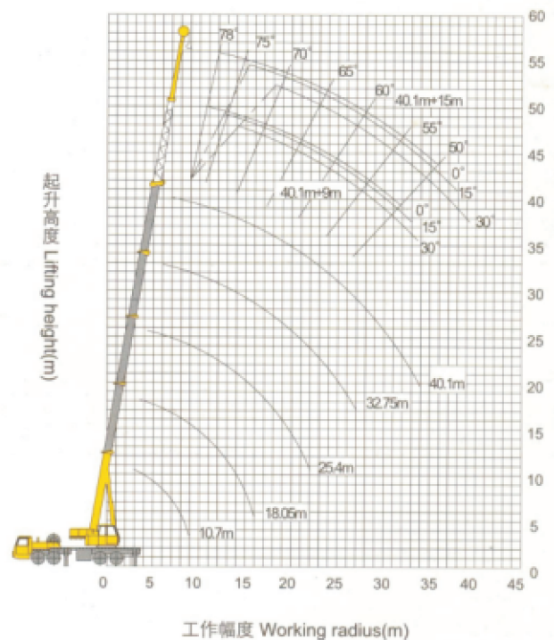
▲ 起升高度曲线 Lifting height curves
