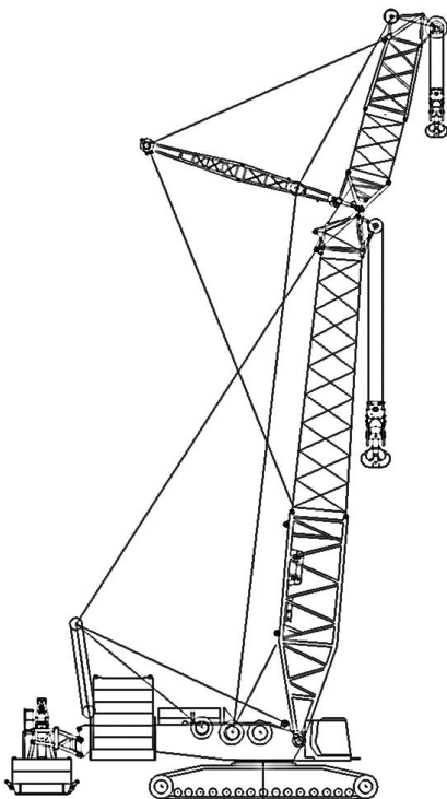
Standard enhanced TBM jib (EHFS)
