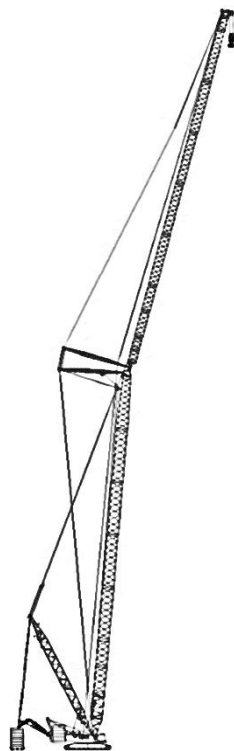
Superlift tower jib (SHW)
