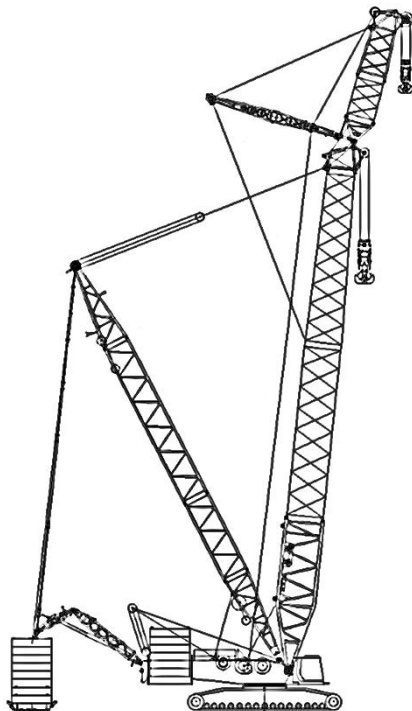
Superlift TBM jib (SHFS)
