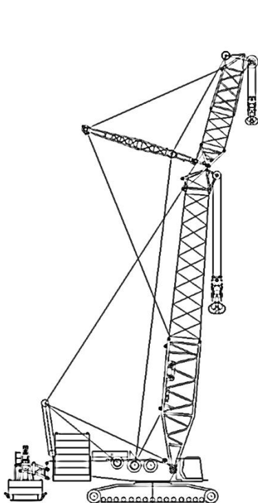
Standard TBM jib (HFS)
